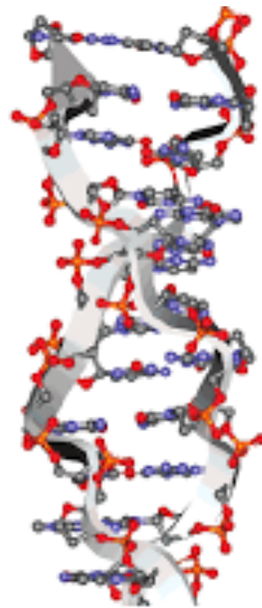
Z-DNA
