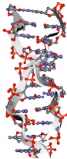
Z-DNA
