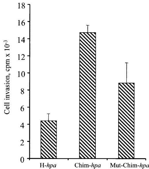
Figure 5. Invasion through Matrigel of cells expressing active vs. inactive heparanase. 3 H-thymidine-labeled Eb cells transfected with H- hpa , chimeric hpa , or Mut-chimeric hpa were incubated ( 1 \times 10^6 cells/mL, 6 h, 37°C, pH 7.4) in RPMI medium supplemented with 0.1% BSA on top of Matrigel-coated filters. After incubation, the upper surface of the filter was wiped free of cells and the extent of cell invasion was detected by counting in a \beta -scintillation counter (Materials and Methods). Each data point is the mean \pm SD of triplicate filters.
